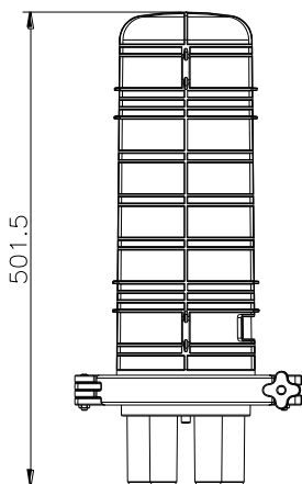
6 round ports
