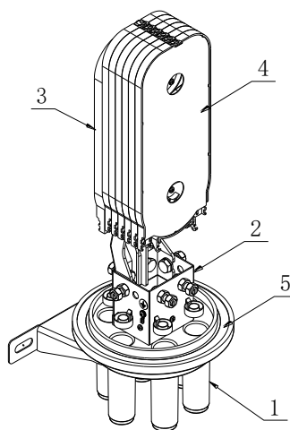
1--base 2--cable fixing board 3--cable storage tray 4--fiber splice tray 5--sealing ring 6--closure body 7--hook
